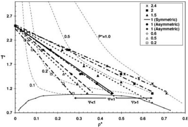
Figure 11. Effect of \Psi on phase behavior of polymer solution.
